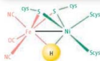
Ni-Fe hydrogenase active site
